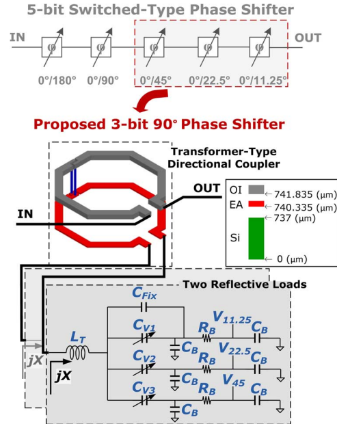
Fig. 1. Conventional 5-bit STPS and the proposed 3-bit 90 phase shifter.
