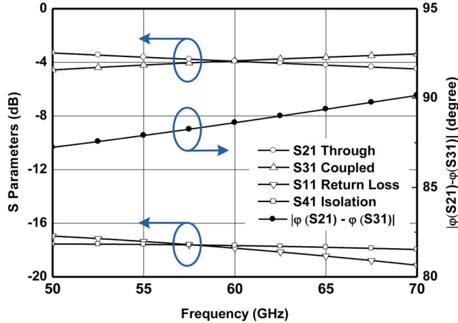
Fig. 2. Simulated performance of the transformer-type directional coupler.
