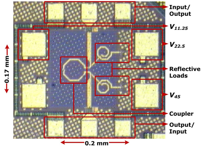
Fig. 3. Micrograph of chip die.
