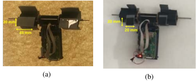
Fig. 9: Adhesion area (a) PDMS with foam backing layer, (b) Micro-Suction with foam backing layer
