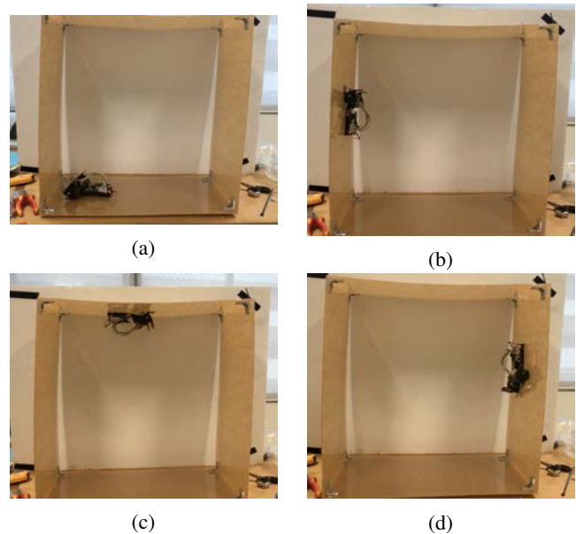
Fig. 11: ORION-II with internal transitions capabilities: (a) Horizontal, (b) Vertical-up, (c) Upside-down, (d) Vertical-down
