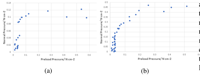
Fig. 4: Normal Pressure versus Preload Pressure for a bilayer foot material (a) PDMS without foam backing layer, (b) PDMS with foam backing layer
