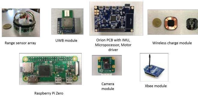
Fig. 6: Electronic components needed for ISR tasks (weight of 67 g)
